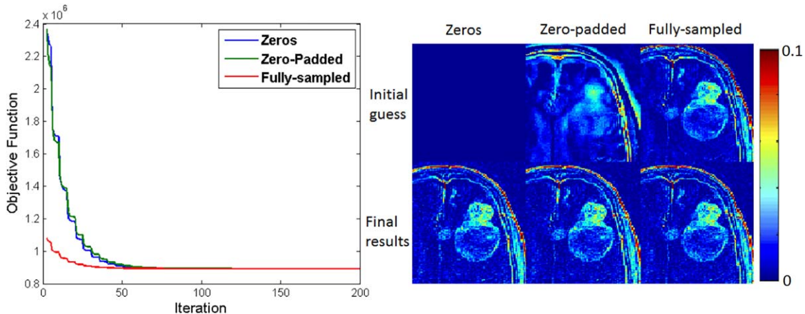
FIG. 2. Objective function versus iteration number for three initial TK parameter estimates (left) and cropped portions of these initial and final TK maps (shown is the K^{\text{trans}} map) at a undersampling rate of 20 \times (right). All initial conditions converged to the same solution. No benefit was observed using a zero-padded k-space relative to a null starting condition.
